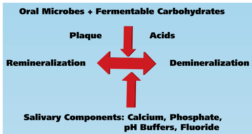
Figure 1. Example of the demineralization-remineralization process in the oral plaque.
