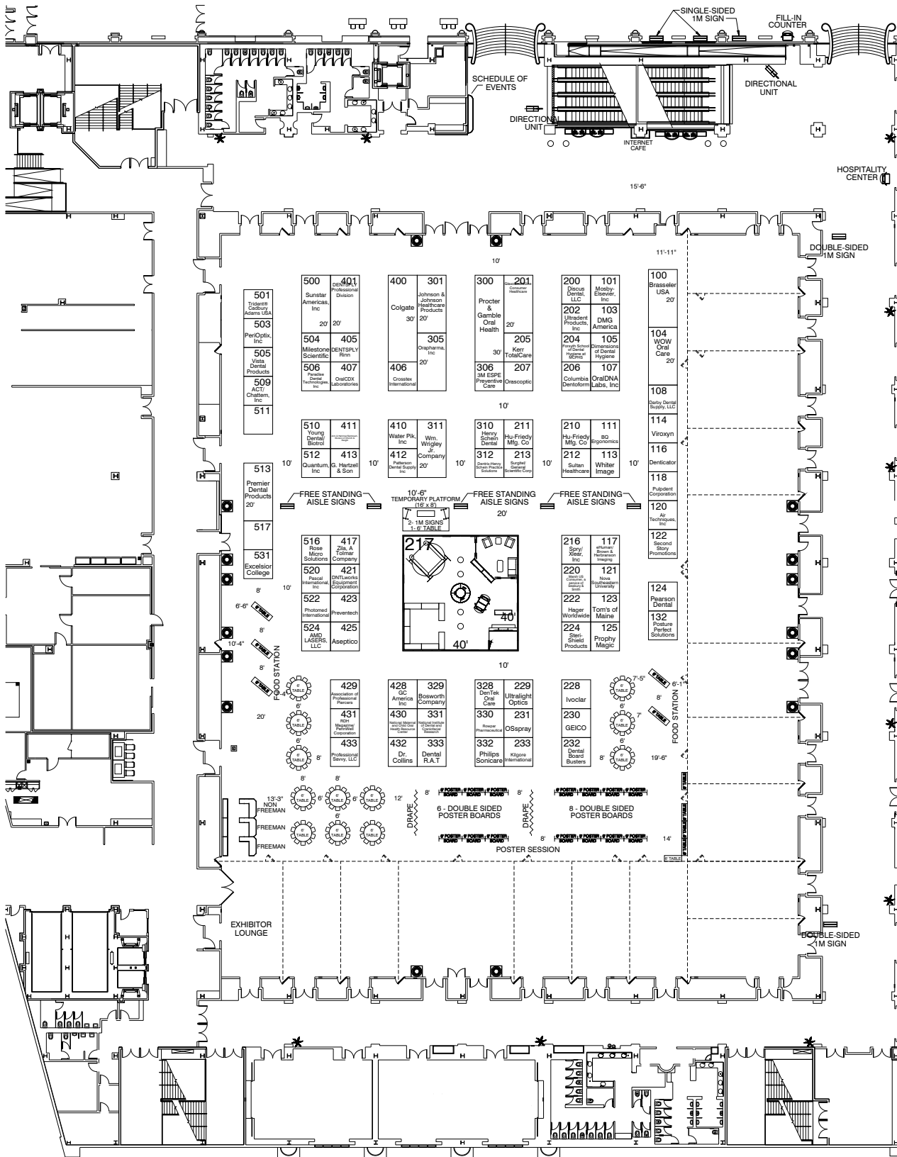
3RD FLOOR, PROMENADE LEVEL SOUTH
